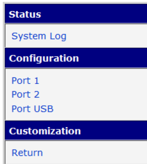
Figure 1: Main menu
